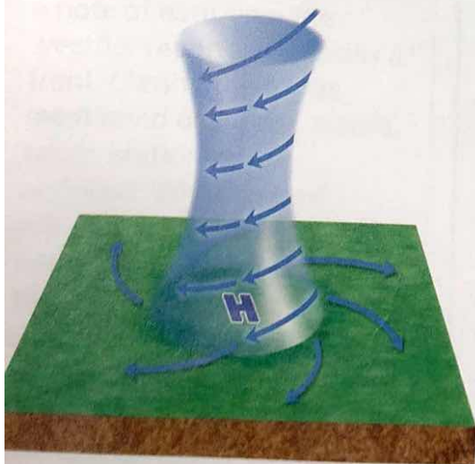
Anticyclone (High)
