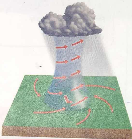
Cyclone (Low)
